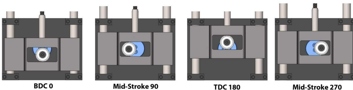
Figure 2: the scotch-yoke movement
