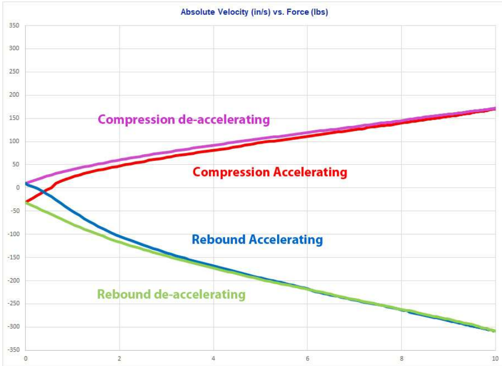
Figure 6: Force vs Absolute Velocity of one cycle
