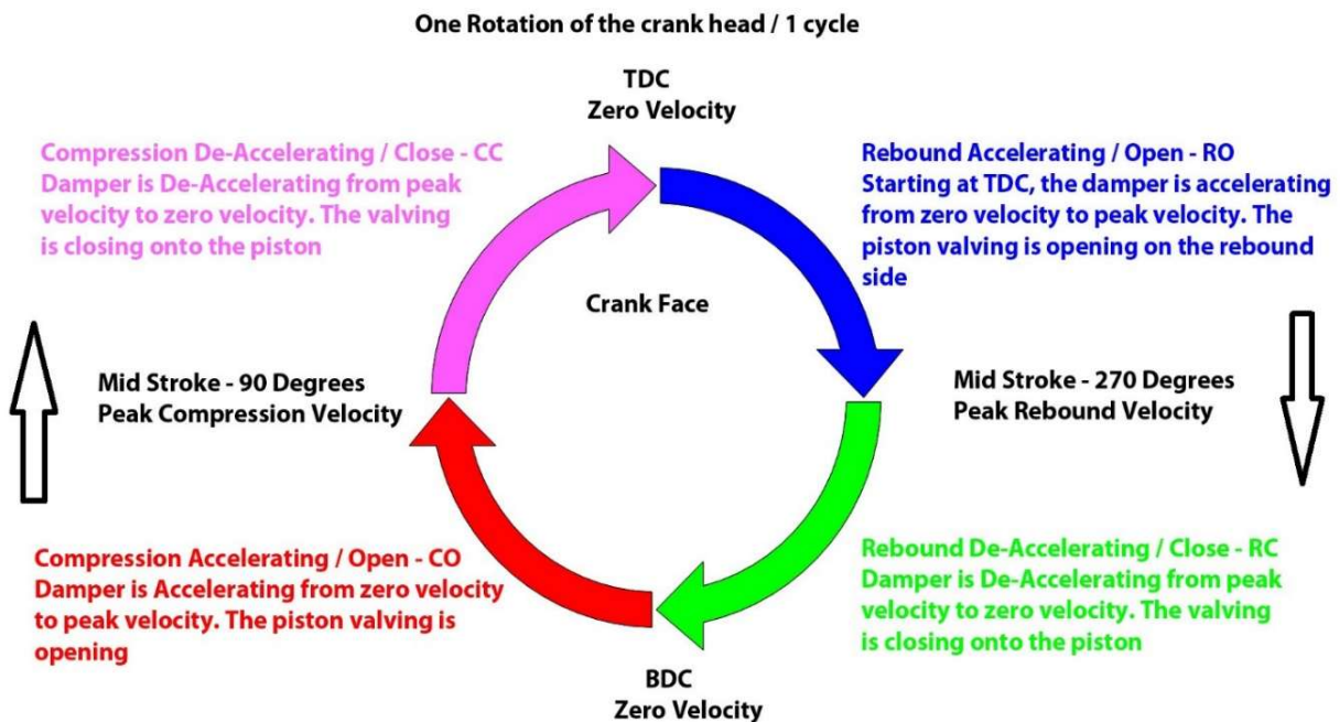
Figure 3: One cycle or rotation of the crank
